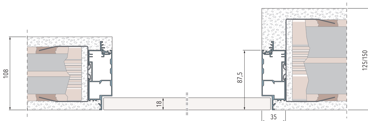
Frame on stud wall, with one or two plasterboard layers and finished according to customer's specifications
