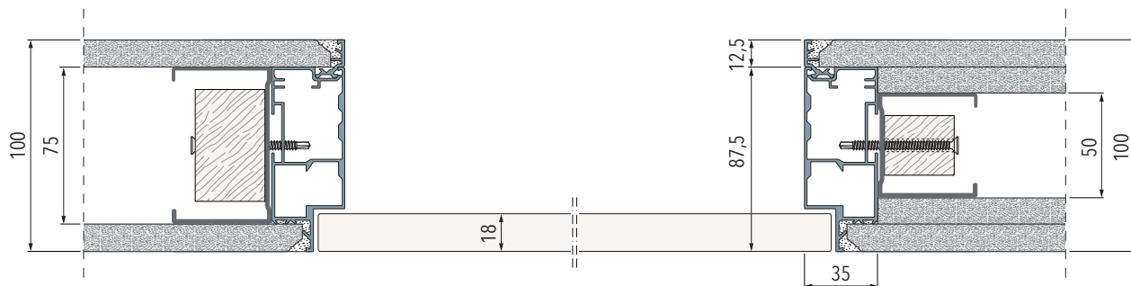
Frame on stud wall, with single or double layer for internal reveal
