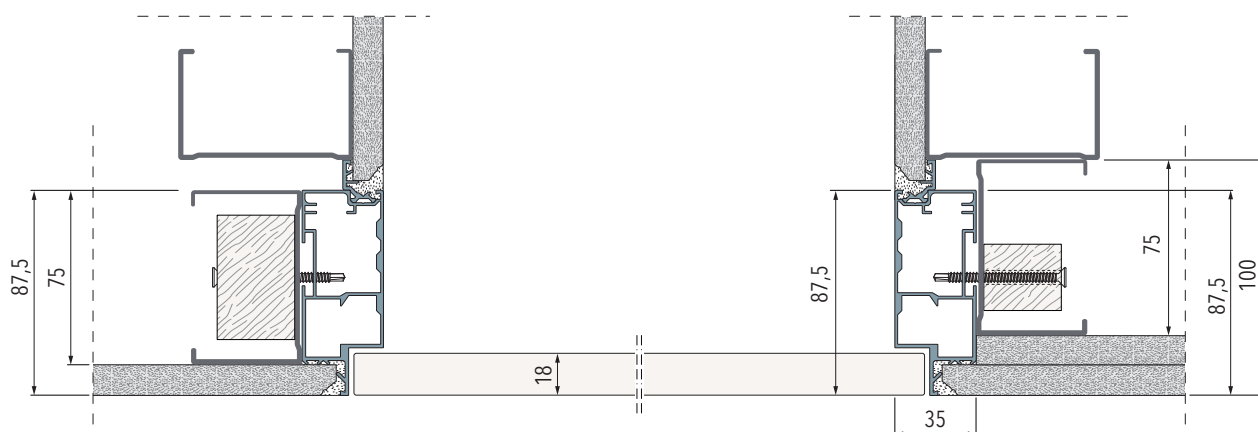
Frame on stud wall, with single or double layer for internal reveal
