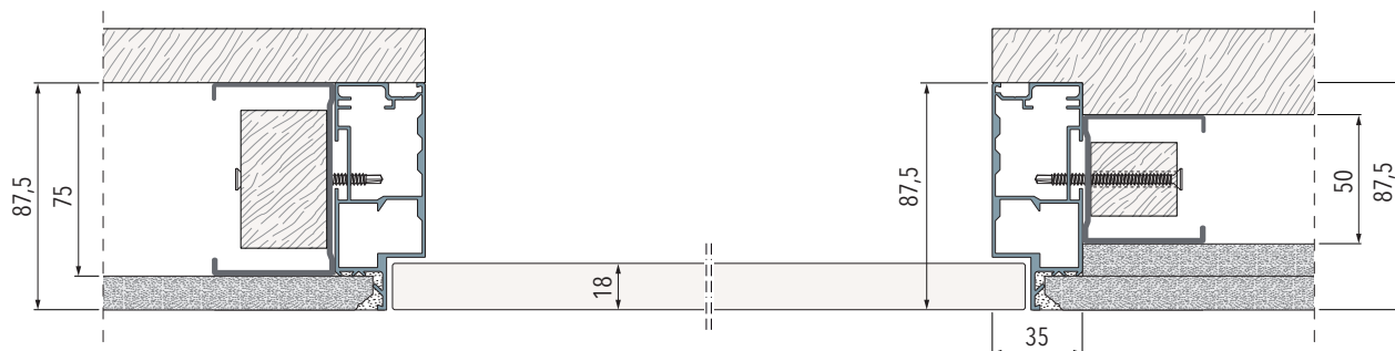
Frame on stud wall, with single or double layer
